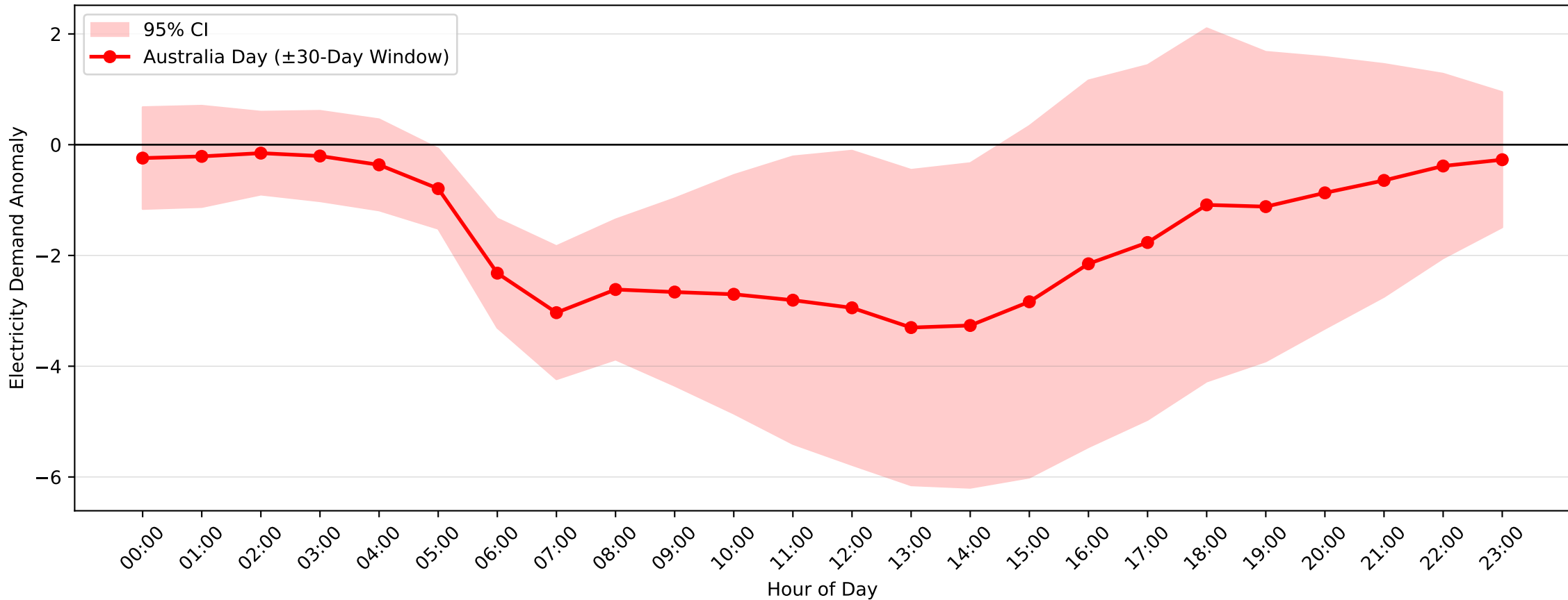
Wyong Demand Anomaly: Australia Day (2004-2017, \pm 30 -Day Window)
